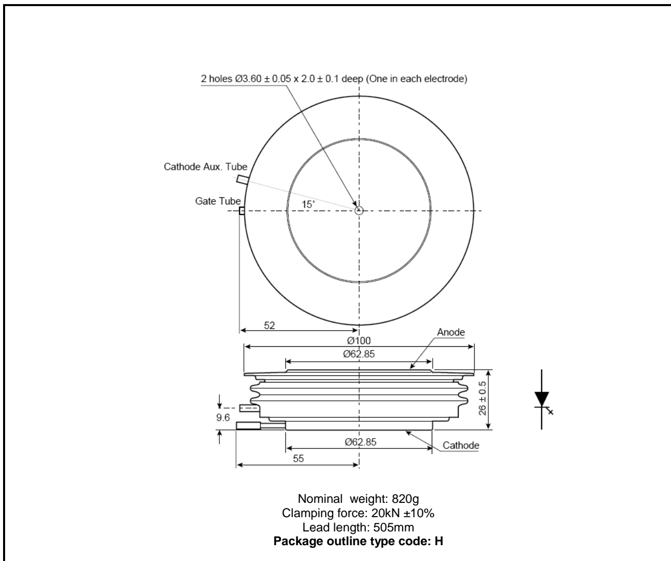
Fig.31 Package outline
